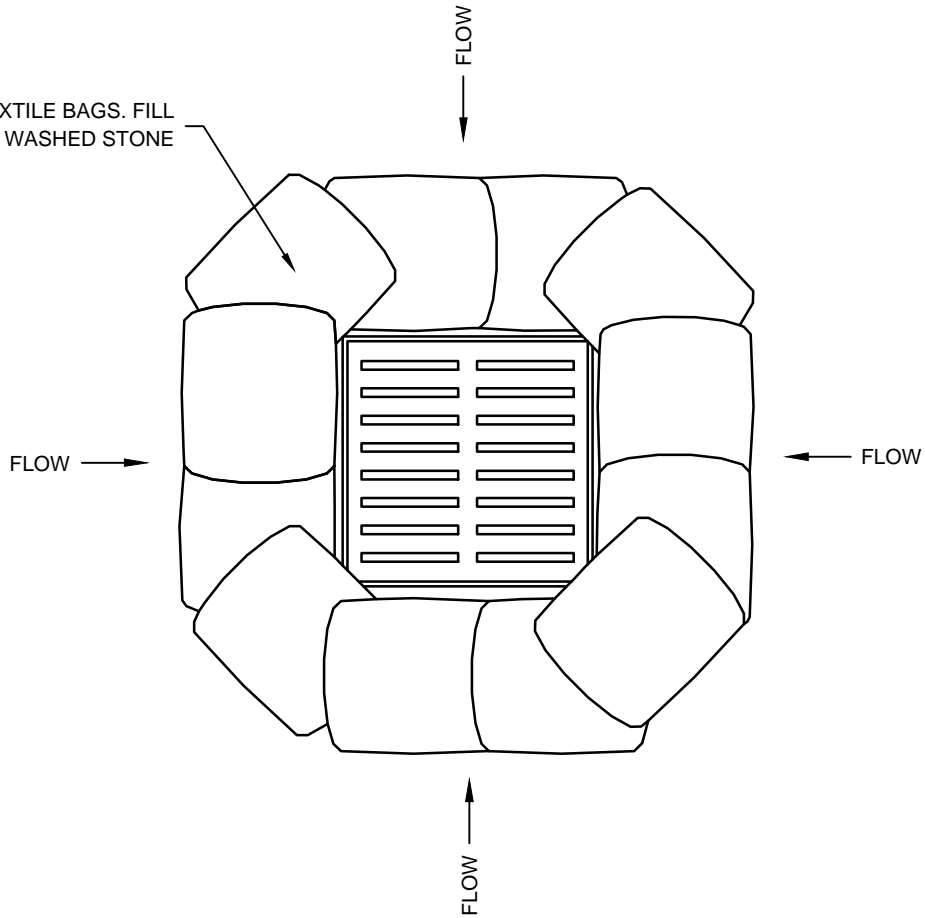
PLAN VIEW
