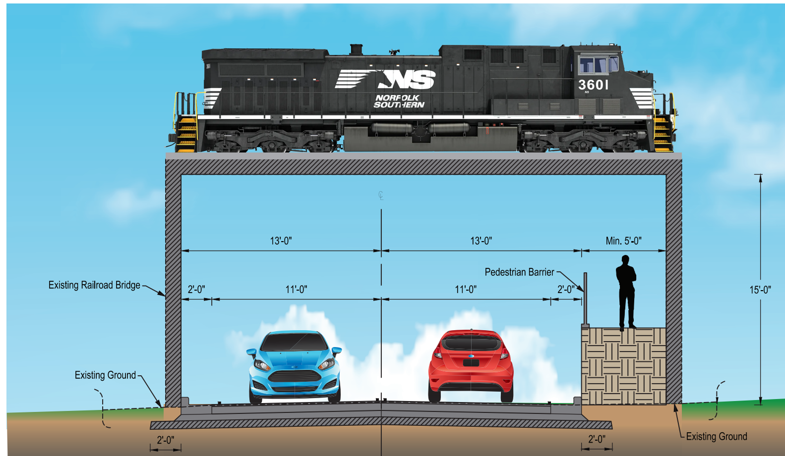
RAILROAD UNDERPASS
