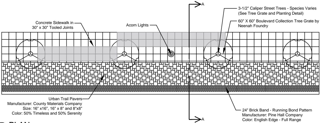
1 PLAN Not to Scale
